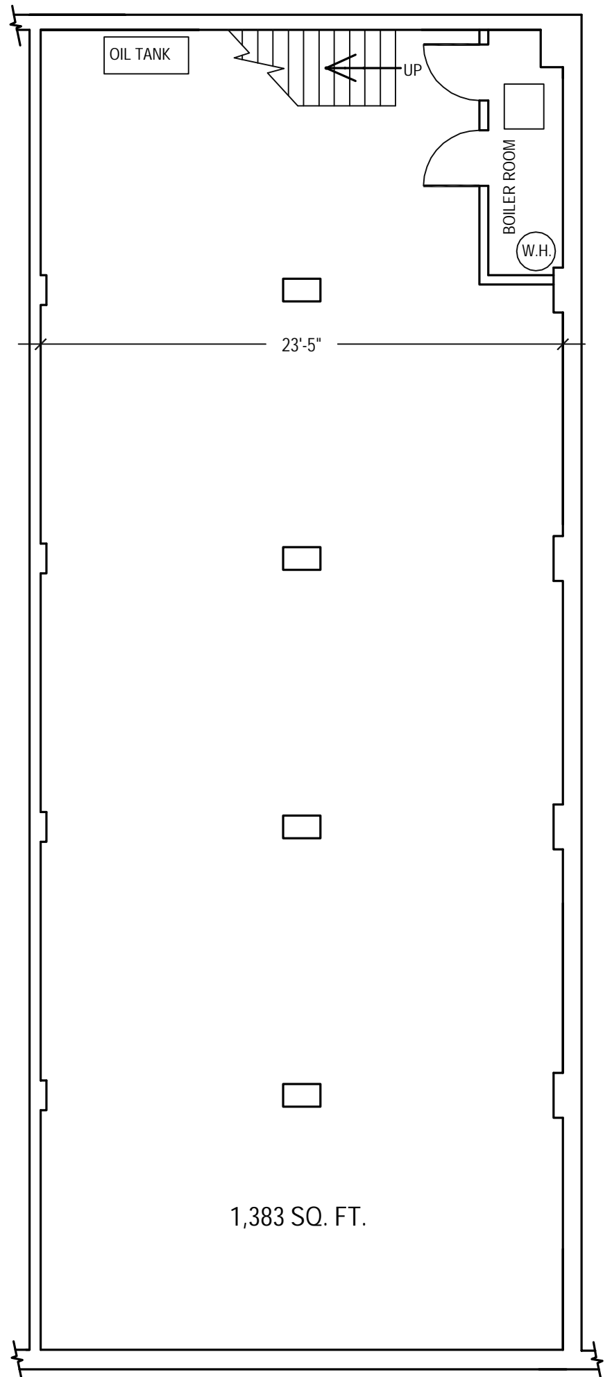
BASEMENT PLAN
